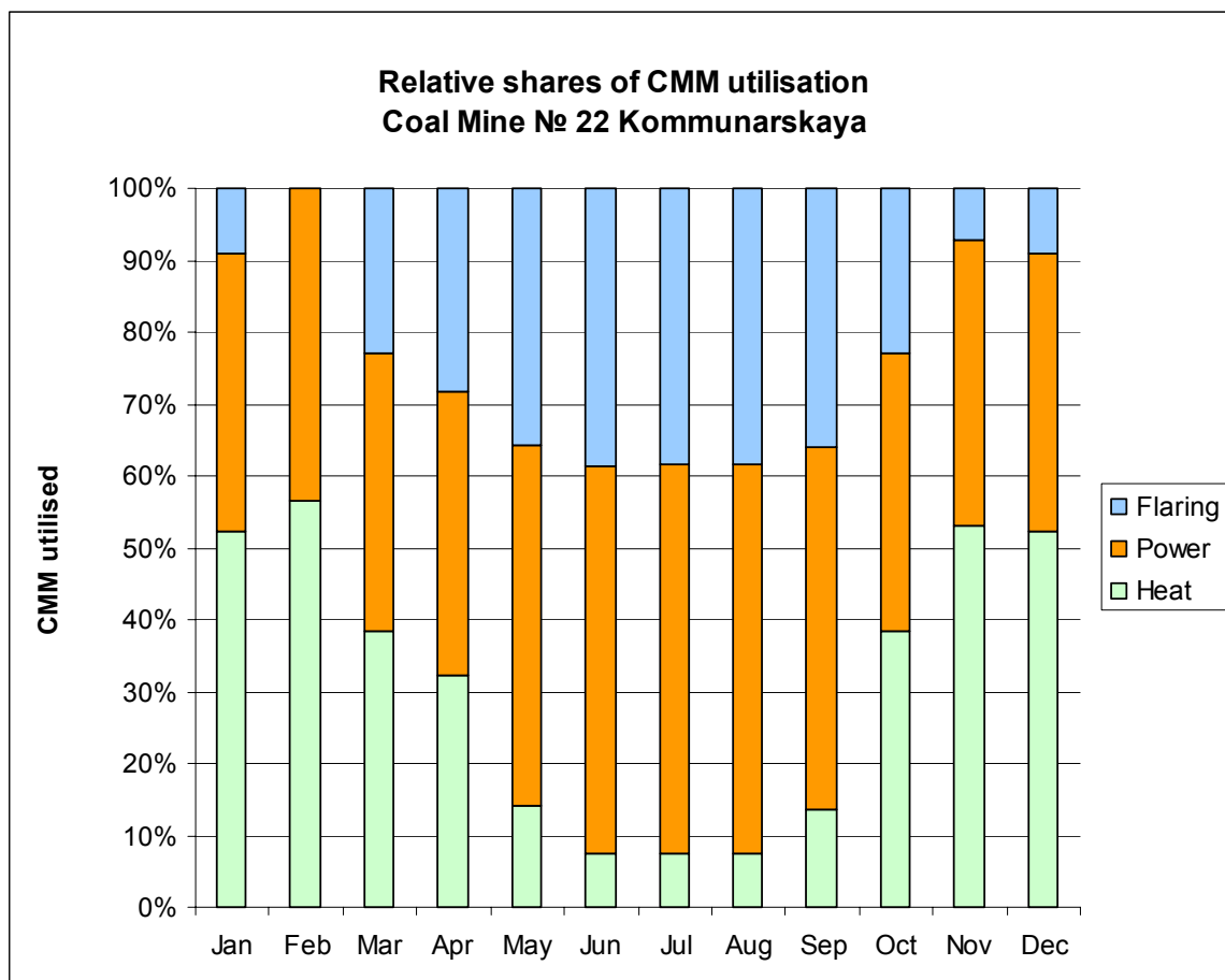
Figure B-1: Relative shares of the CMM utilisation by flaring, power and heat generation. The figure shows exemplary the prospected values for the years 2009-2017
