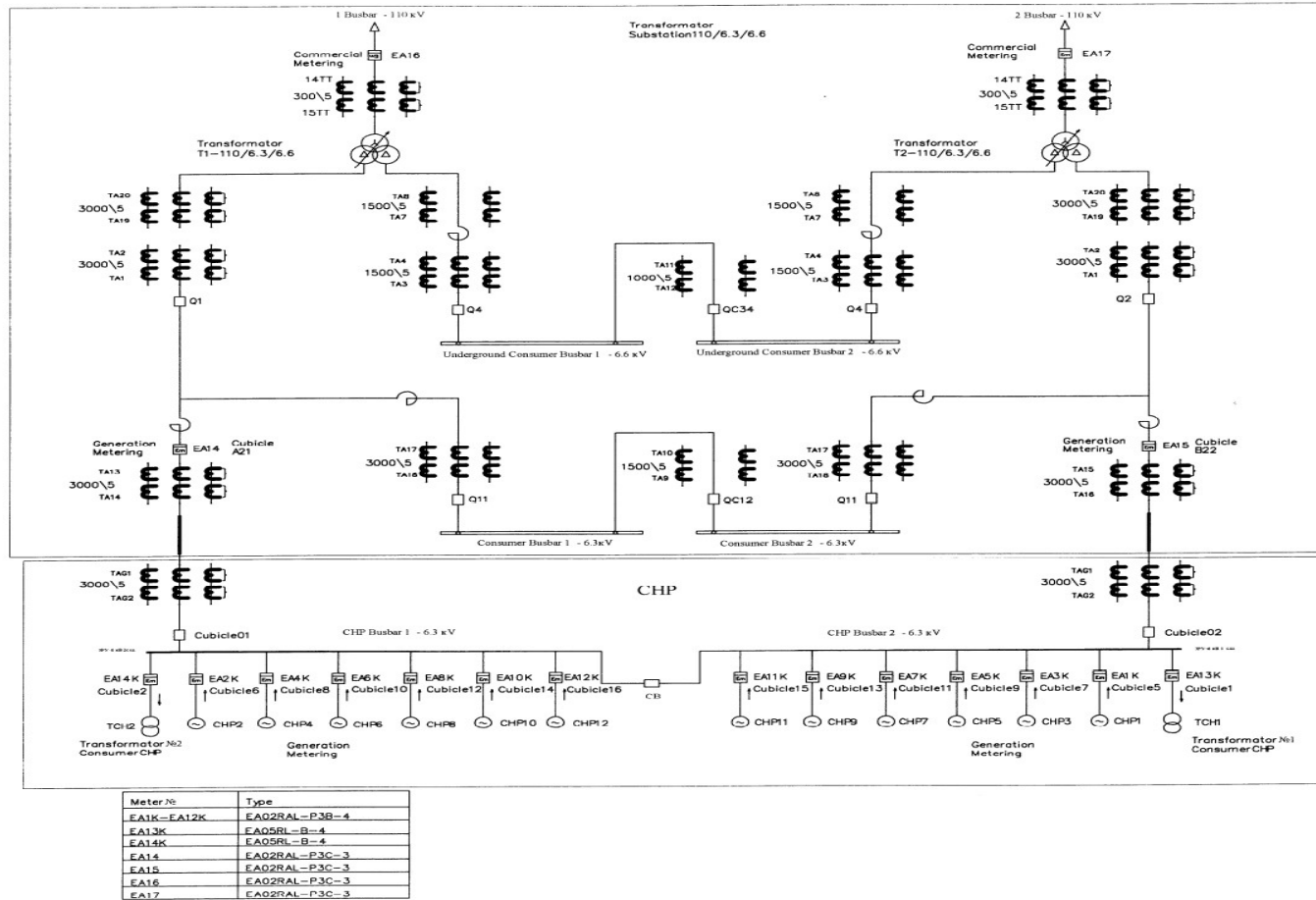
Electricity Metering Scheme for Vostochnaya CHP Facility
