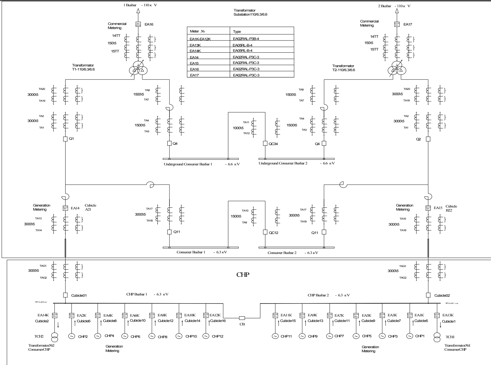
Figure 2: Electricity Metering Scheme for Vostochnaya CHP Facility after changes put on 04.03.2009
