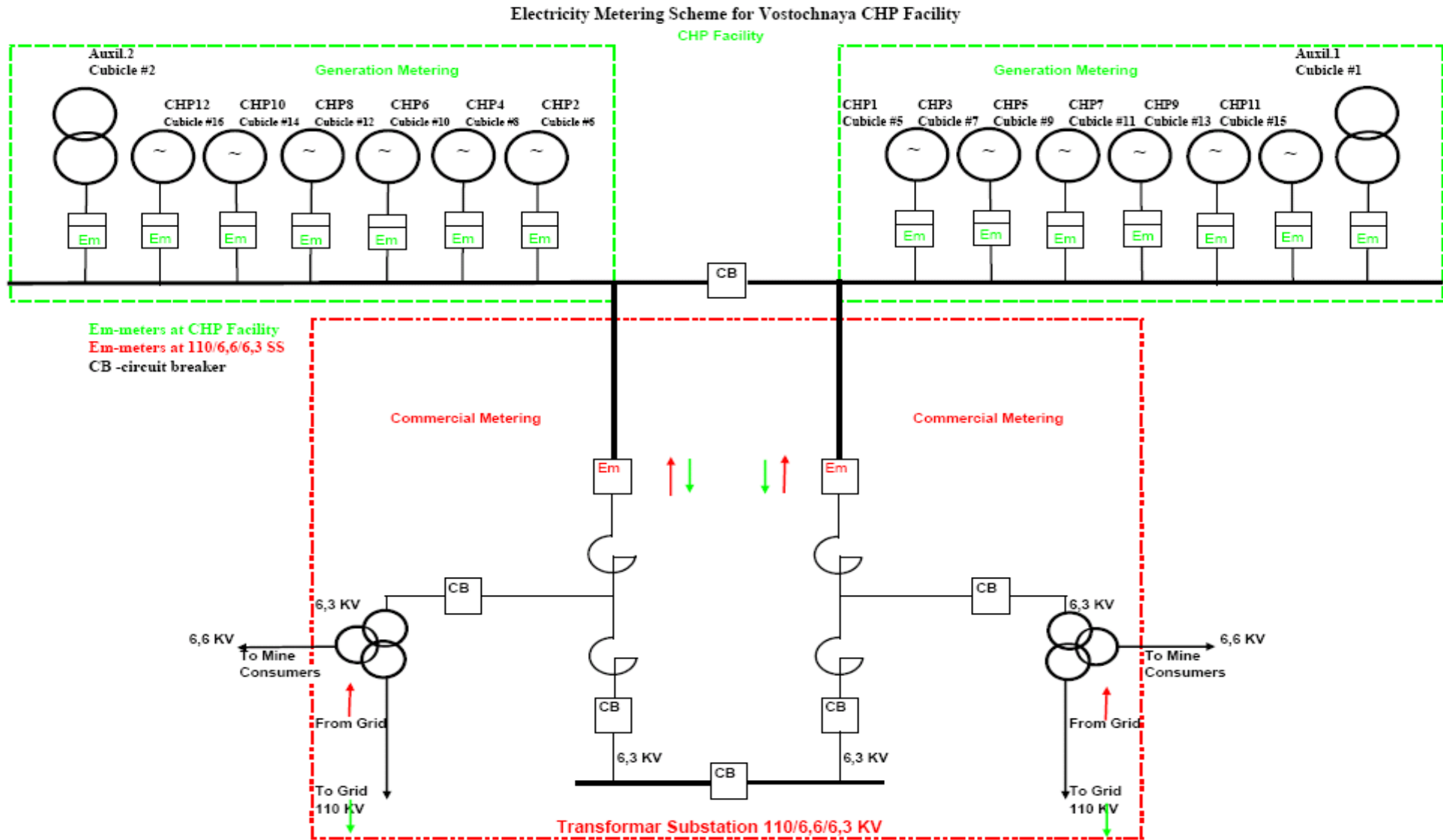
Figure 1: Electricity Metering Scheme for Vostochnaya CHP Facility
