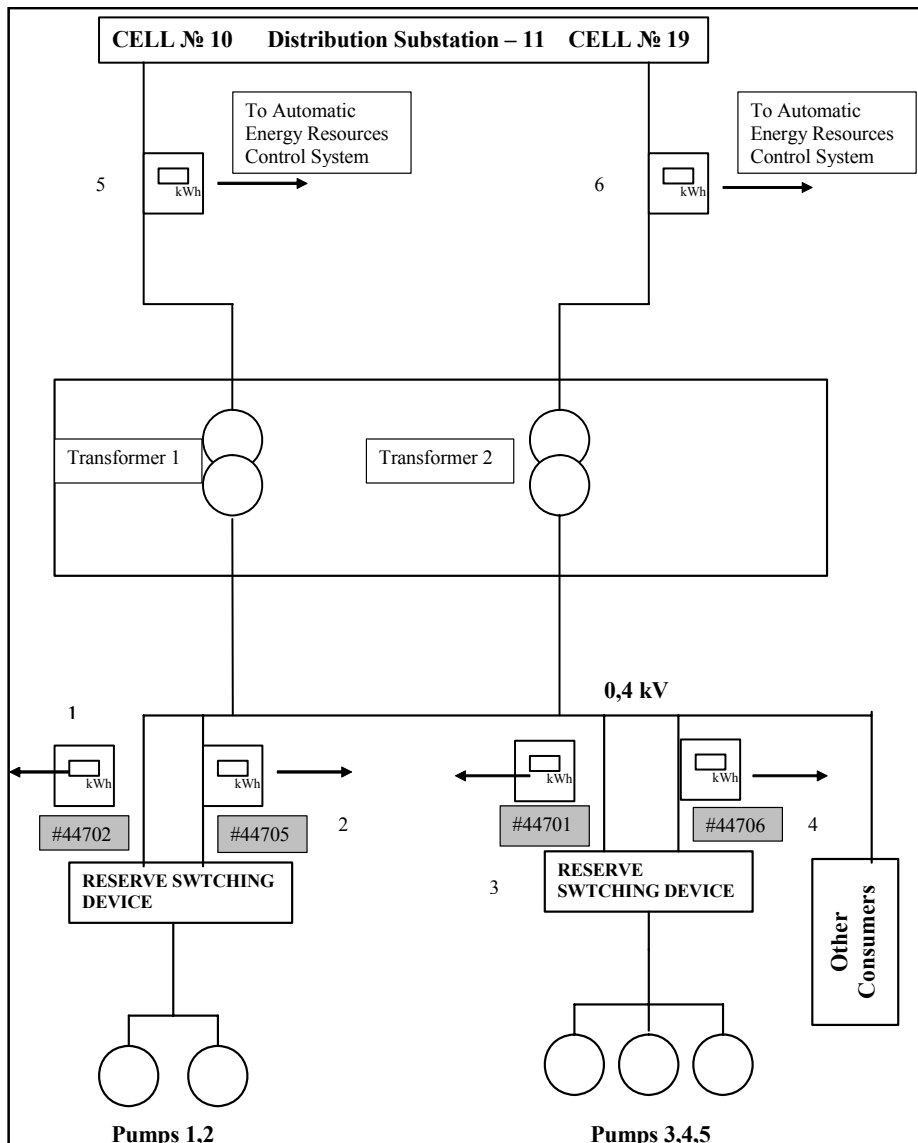
Figure 3. Electricity metering system at VD
