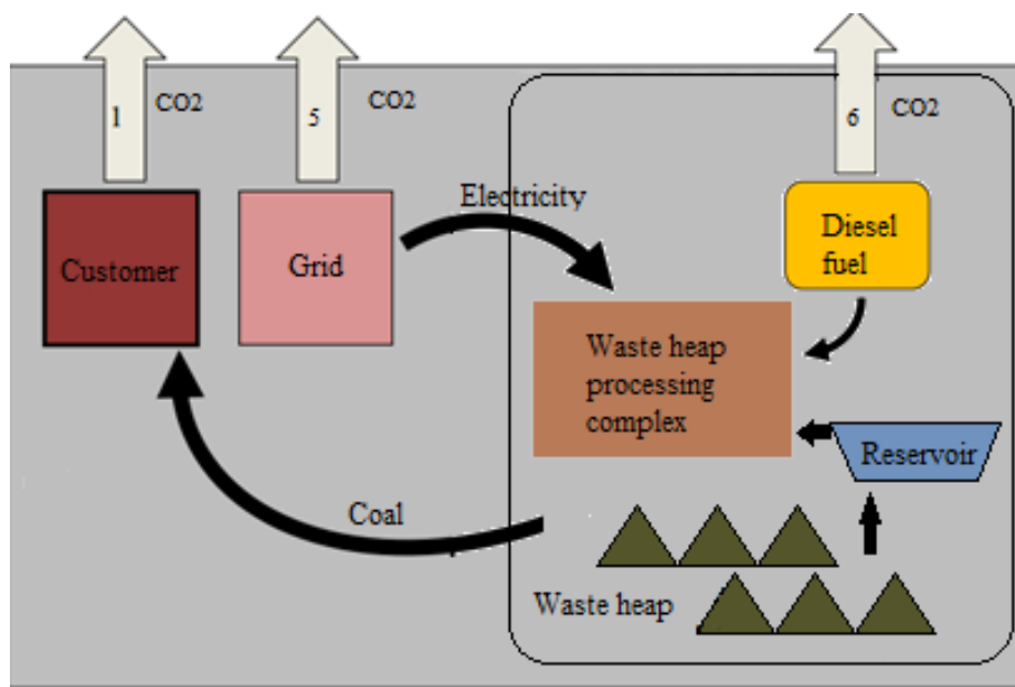
Fig.7 Project boundaries in the project scenario
