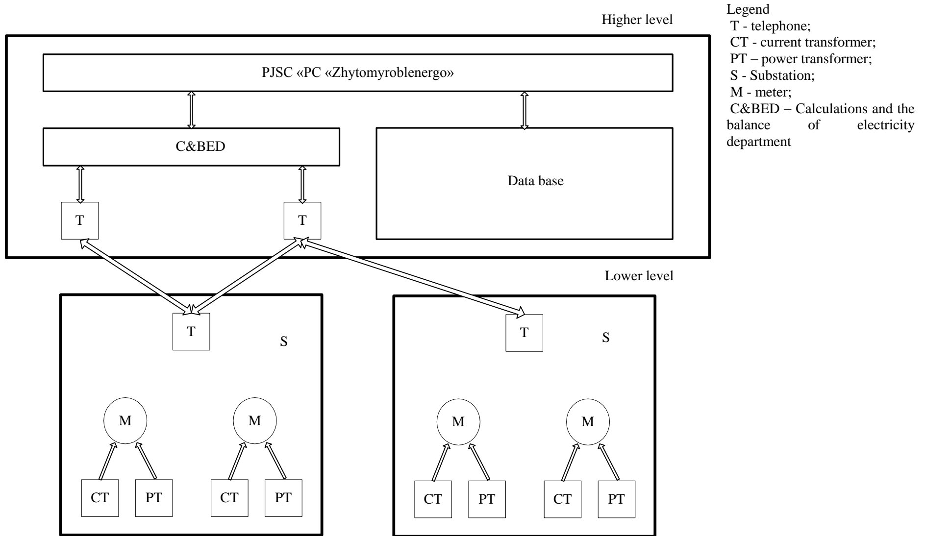
Figure 14. Scheme of data collection prior to implementation of the automated system of electricity consumption commercial records (ASECCR)
