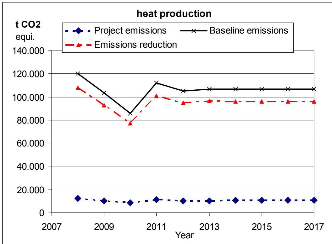
Figure E-3 - Baseline emissions, project emissions and emissions reduction; heat generation units, both crediting periods
