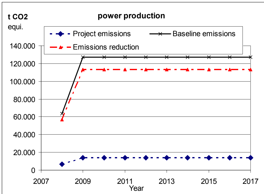
Figure E-4 - Baseline emissions, project emissions and emissions reduction; power generation units, both crediting periods
