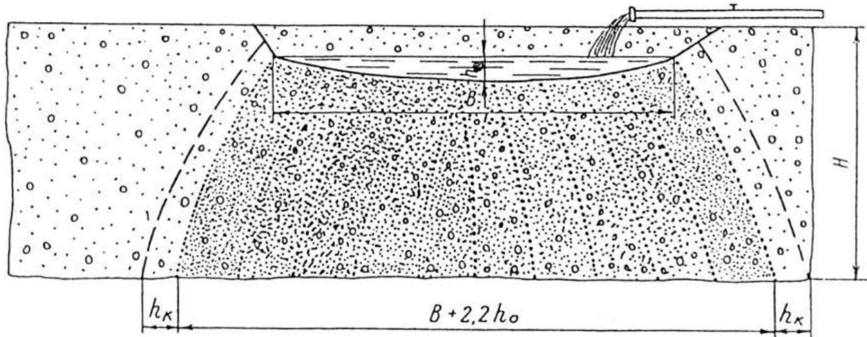
Fig. 4. Scheme of waste heaps wetting through free antipyrogen filtration.
