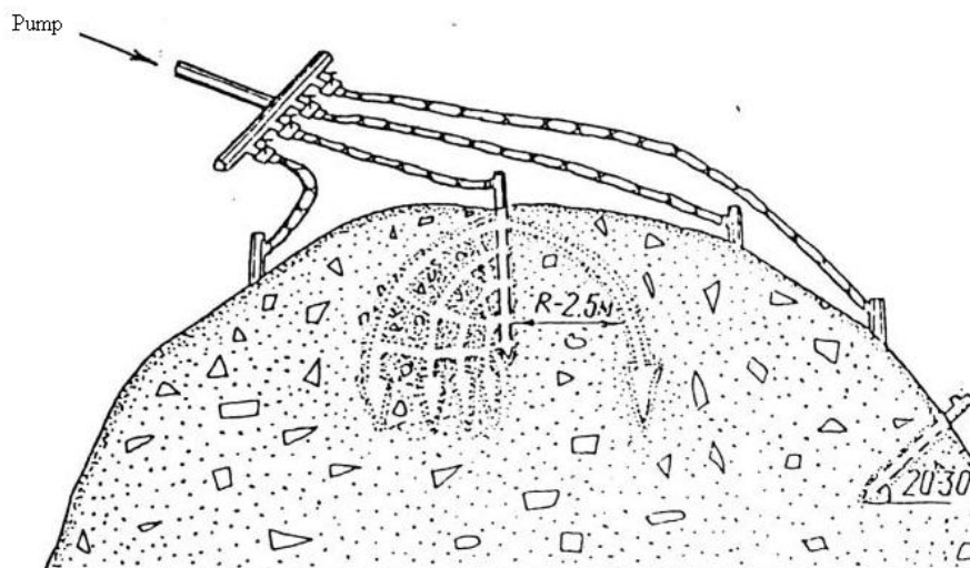
Fig.3. Scheme of antipyrogen injection applying the perforated tubes.
