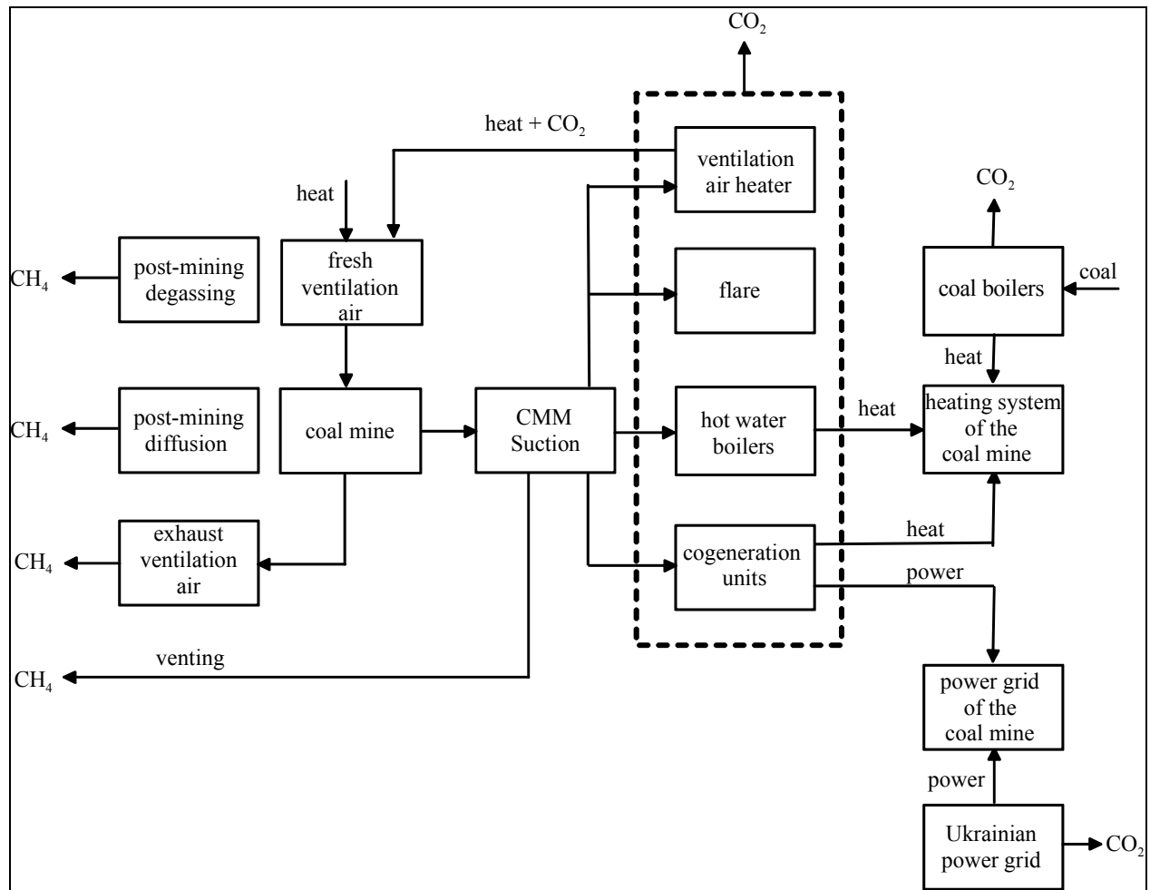
Figure B-3: Project boundary
