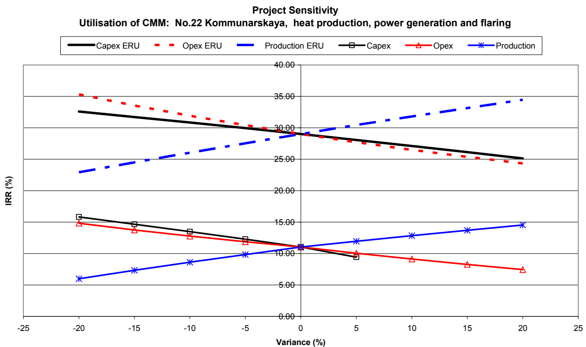
Figure B-2: Sensitivity analysis of economic indicators of the project
