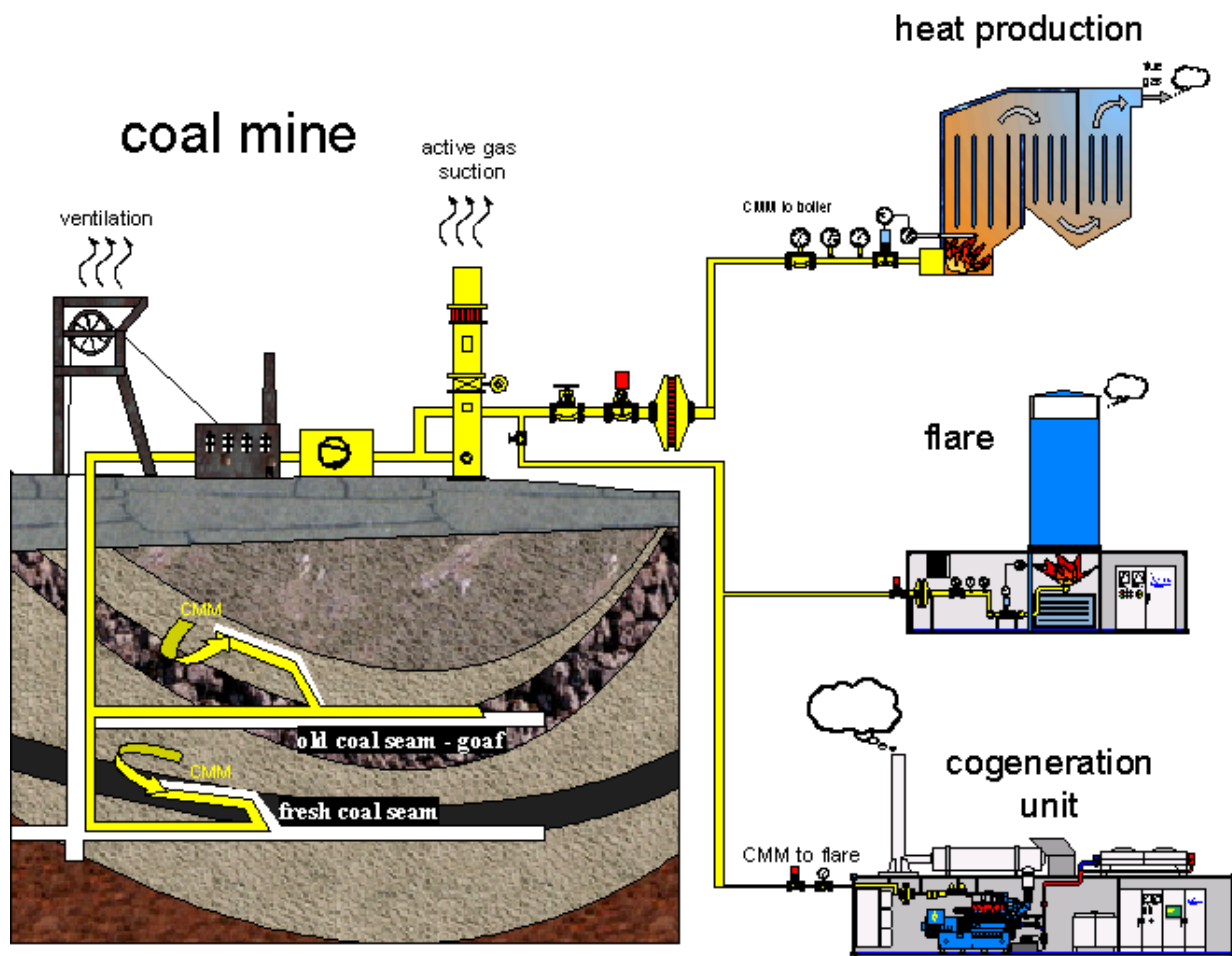
Figure A- 2: General scheme of the installation with main project components
