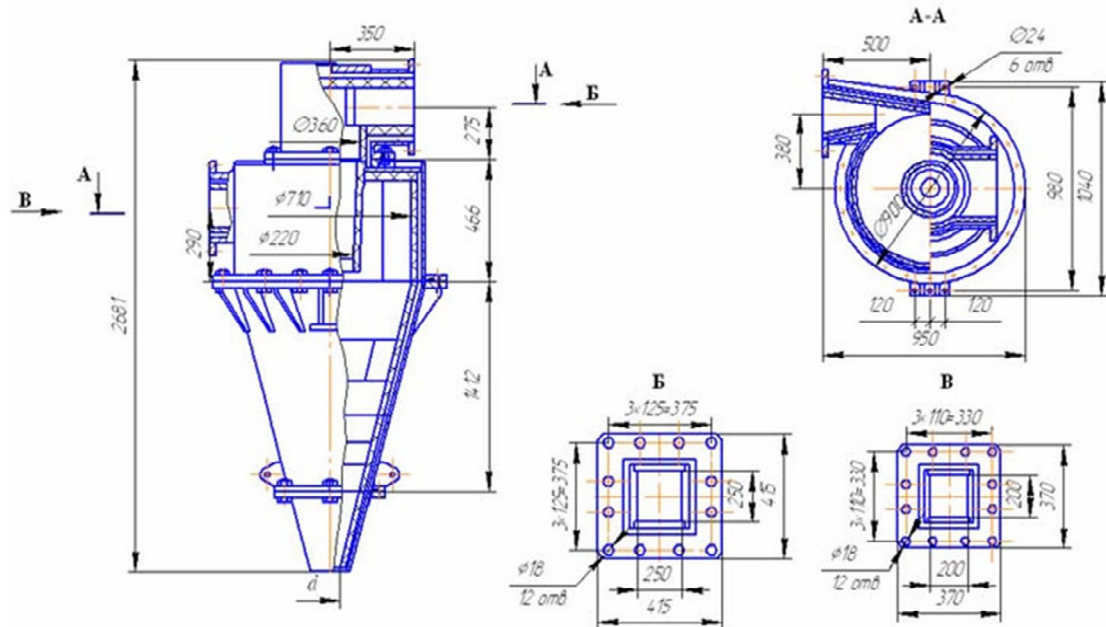
Figure 4 – Overall dimensions and connecting nodes of hydrocyclone GT-500
