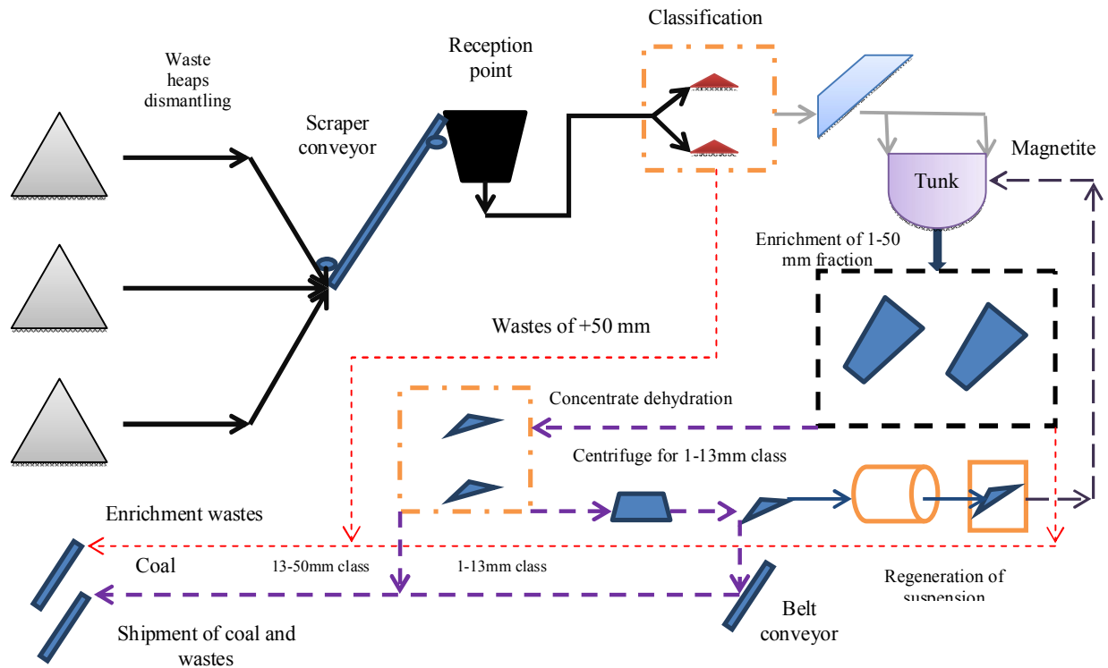
Figure 3 – General flowsheet of the process of carbonaceous rock enrichment
