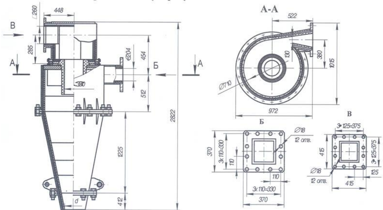
Figure 7 - Hydrocyclone GT-710
