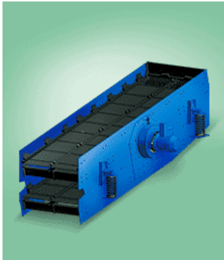
GIL-31 GLKV-1500 Fig.3 Project activity equipment. Classification screens
